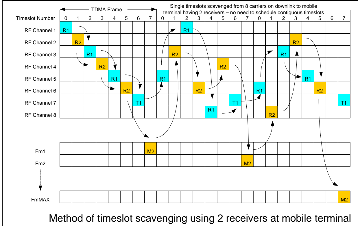
Figure 7: Optimization of Timeslot Usage Example
