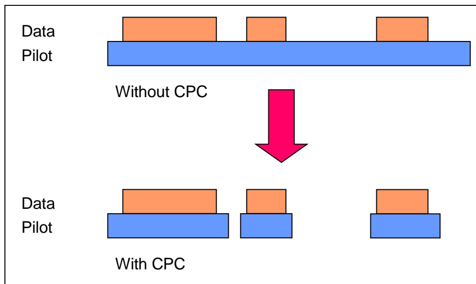
Figure 32: Continuous Packet Connectivity
