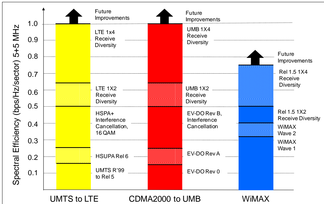
Figure 18: Comparison of Uplink Spectral Efficiency 70
