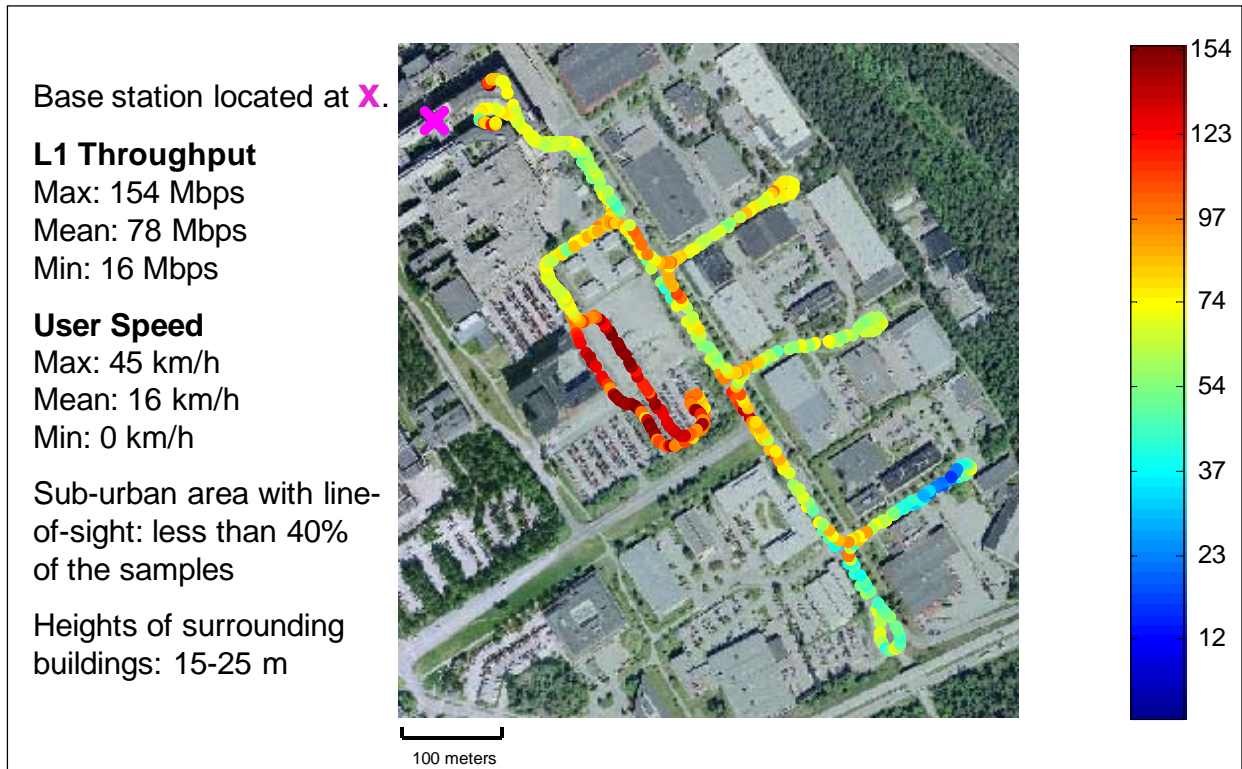
Figure 14: LTE Measured Throughput in Test Network 64
