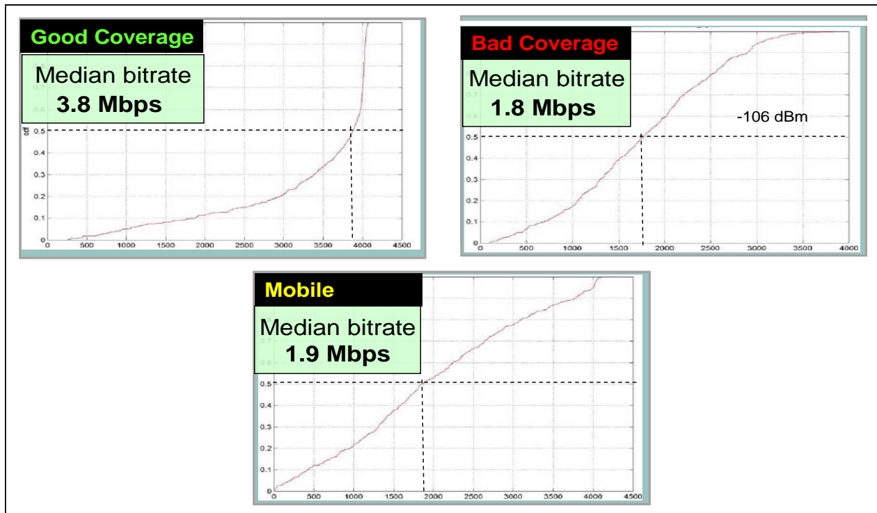
Figure 12: HSDPA Performance of a 7.2 Mbps Device in a Commercial Network 59
