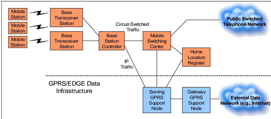
Figure 21: GSM/GPRS/EDGE Architecture
