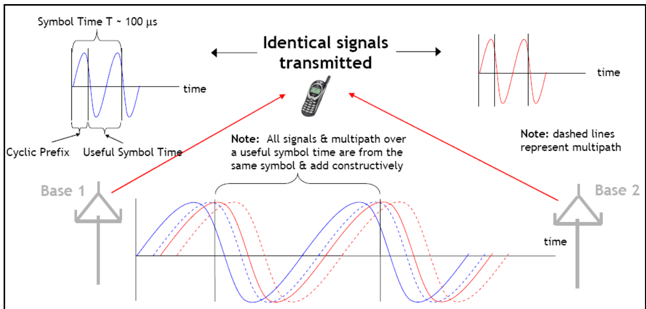
Figure 40: OFDM Enables Efficient Broadcasting
