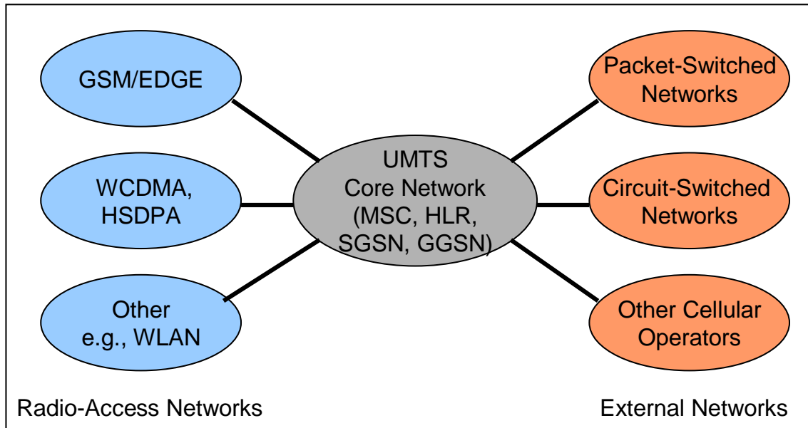
Figure 28: UMTS Multiradio Network
