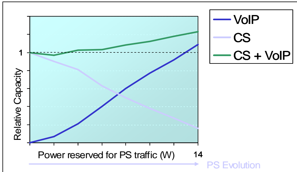
Figure 36: Ability for UMTS to Support Circuit and Packet Voice Users 100
