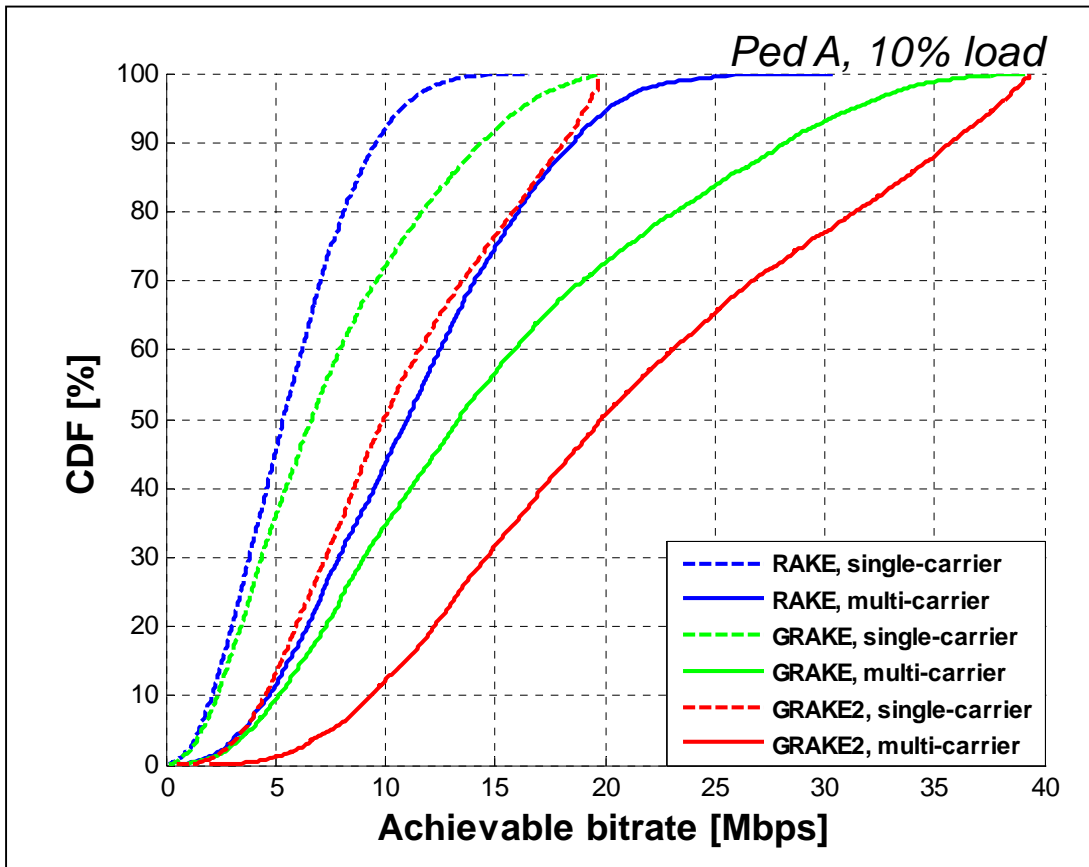
Figure 33: Dual-Carrier Performance 97
