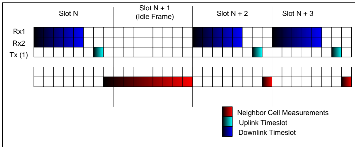
Figure 23: Evolved EDGE Two-Carrier Operation 85
