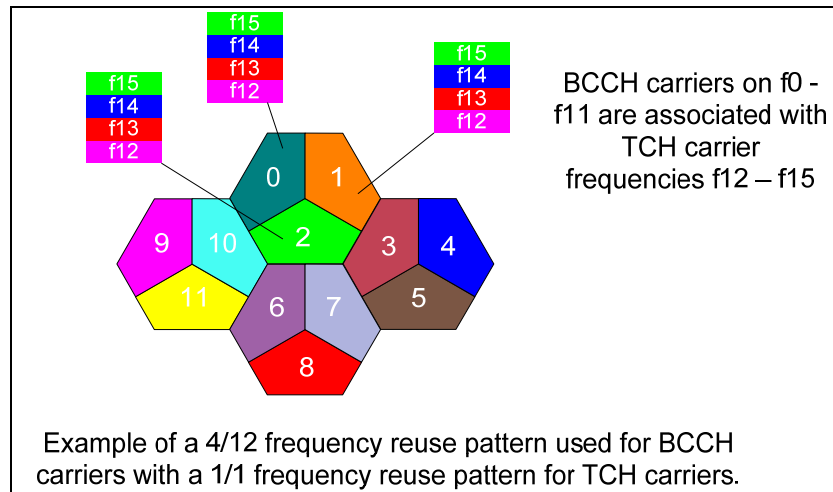
Figure 27: Example of 4/12 Frequency Reuse with 1/1 Overlay 89
