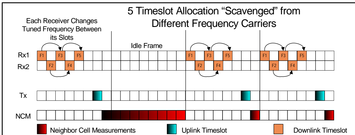
Figure 26: Optimization of Timeslot Usage Example 88
