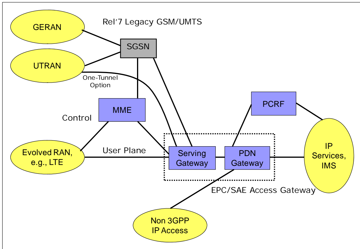
Figure 41: EPC/SAE Architecture
