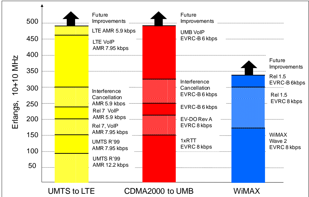
Figure 19: Comparison of Voice Spectral Efficiency 72
