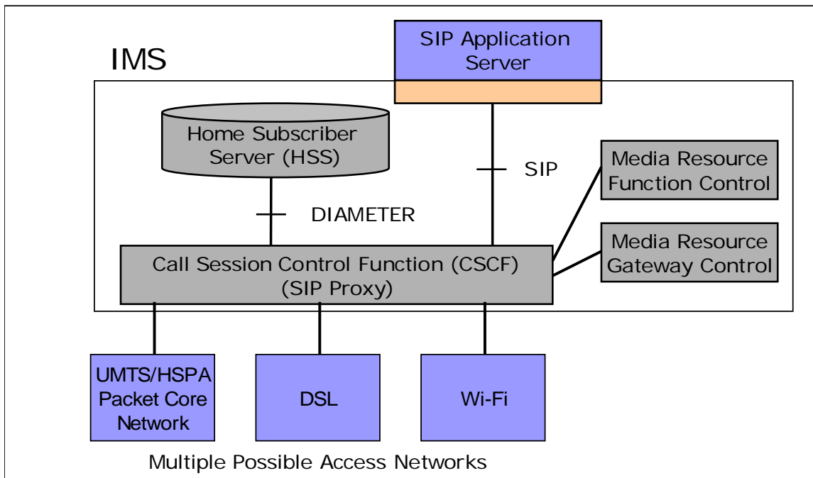
Figure 39: IP Multimedia Subsystem
