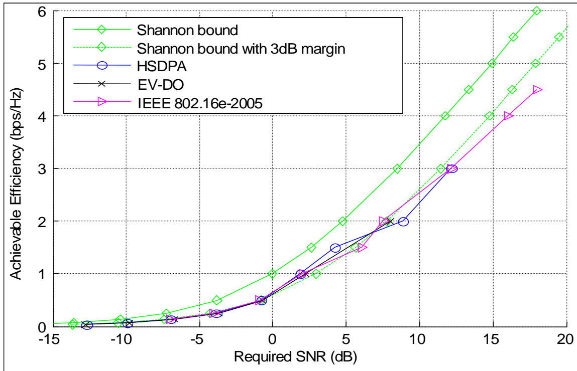
Figure 16: Performance Relative to Theoretical Limits for HSDPA, EV-DO, and IEEE 802.16e-2005 66
