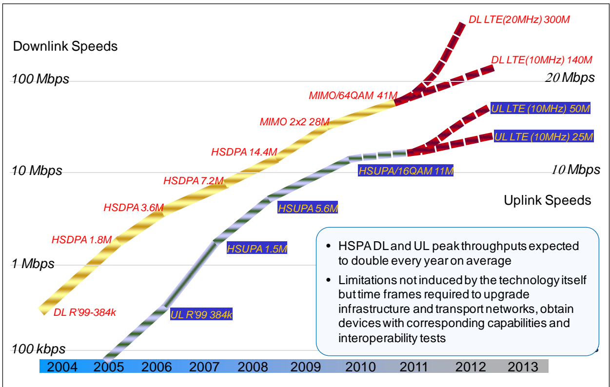
Figure 8: Peak Rates for Downlink and Uplink Over Time 32
