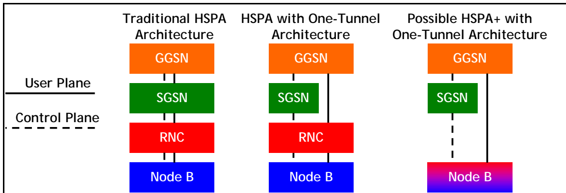
Figure 34: HSPA One-Tunnel Architecture 98
