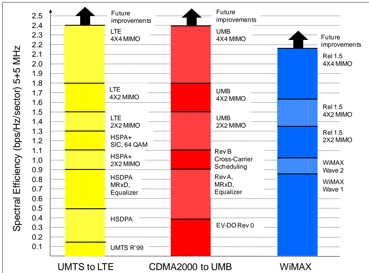
Figure 17: Comparison of Downlink Spectral Efficiency 67
