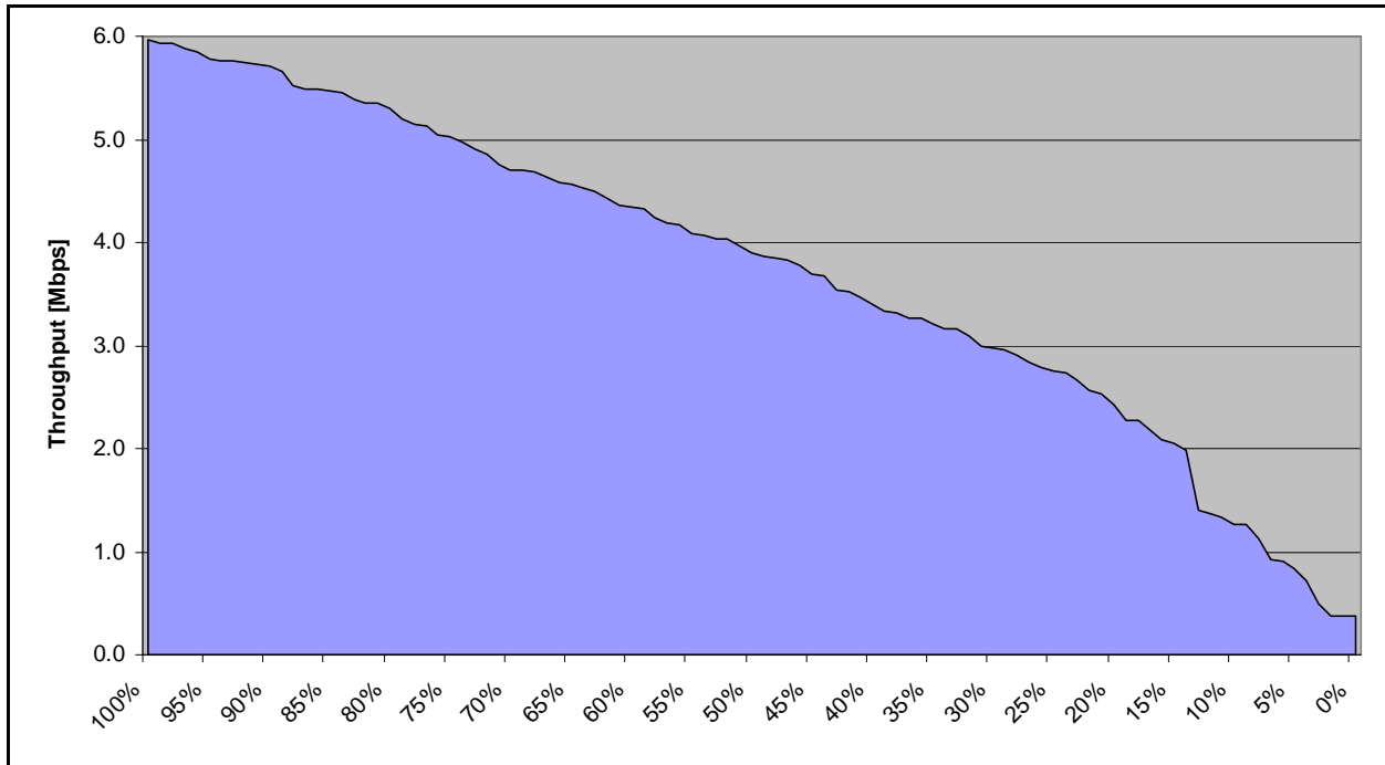
Figure 11: HSDPA Throughput Distribution in Deployed Networks 58
