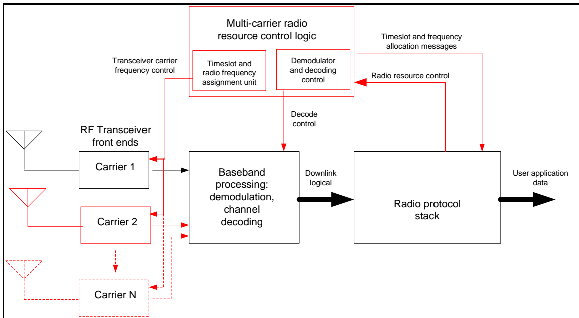
Figure 24: EDGE Multi-Carrier Receive Logic – Mobile Part 86
