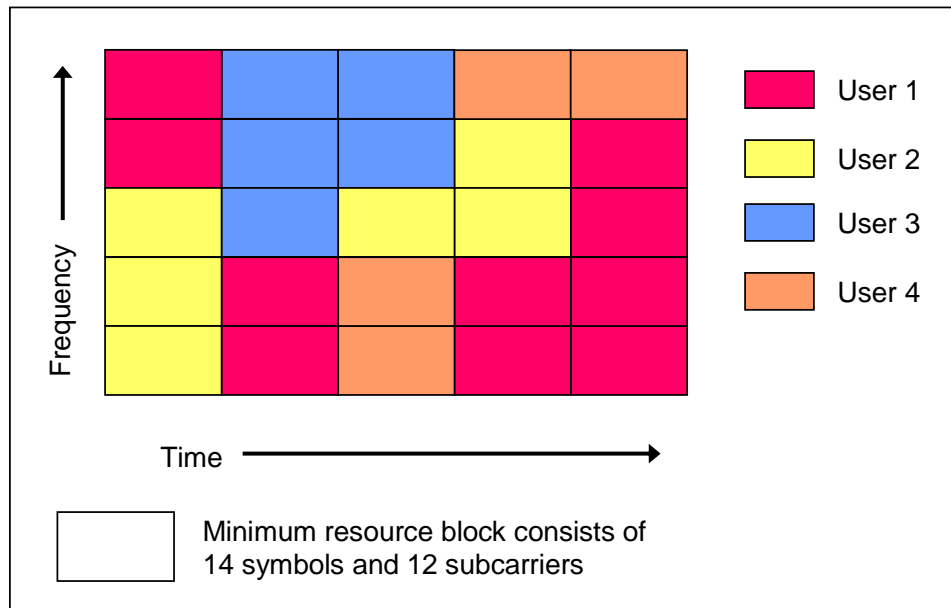
Figure 38: LTE OFDMA Downlink Resource Assignment in Time and Frequency
