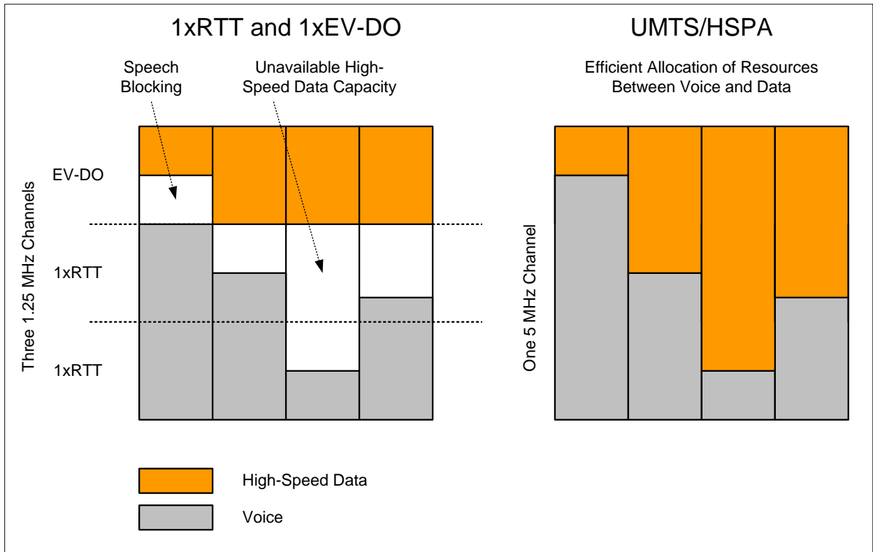
Figure 10: Radio Resource Management 1xRTT/1xEV-DO versus UMTS/HSPA
