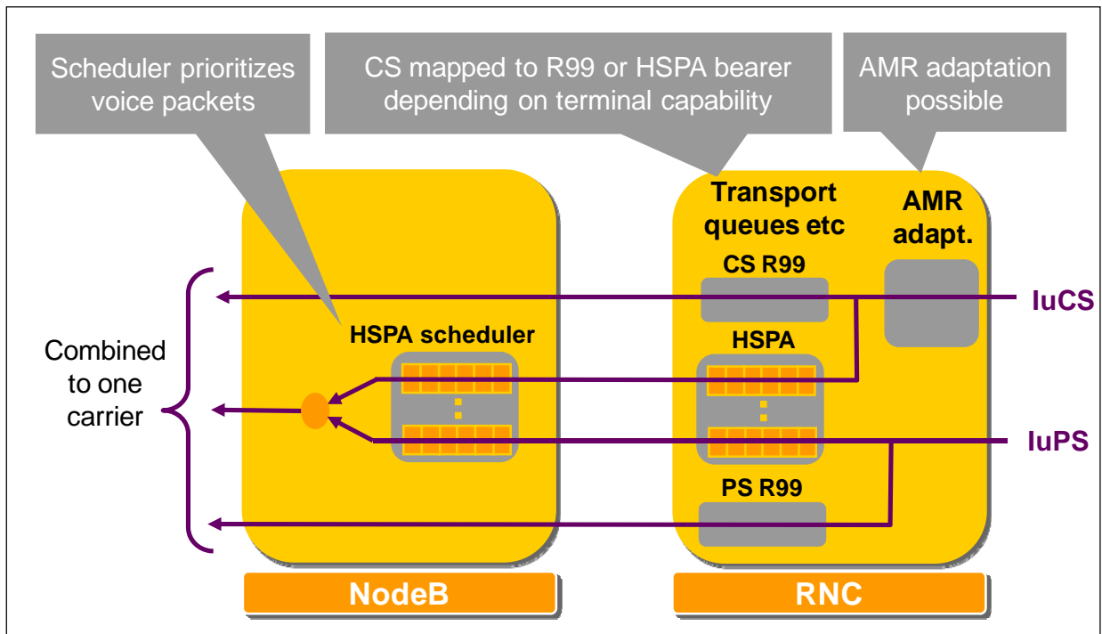
Figure 35: Implementation of HSPA CS Voice 99
