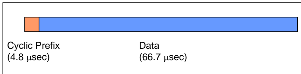
Figure 37: OFDM Symbol with Cyclic Prefix
