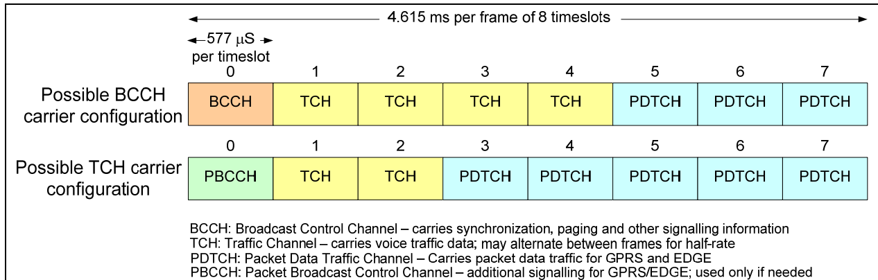
Figure 22: Example of GSM/EDGE Timeslot Structure 82
