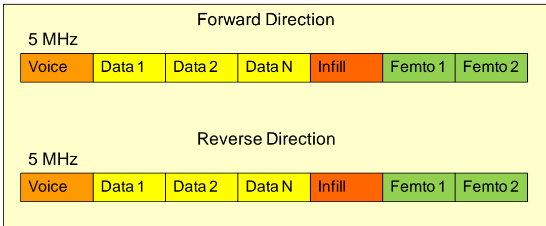
Figure 8: Ideal Radio Channel Deployment for HSPA
