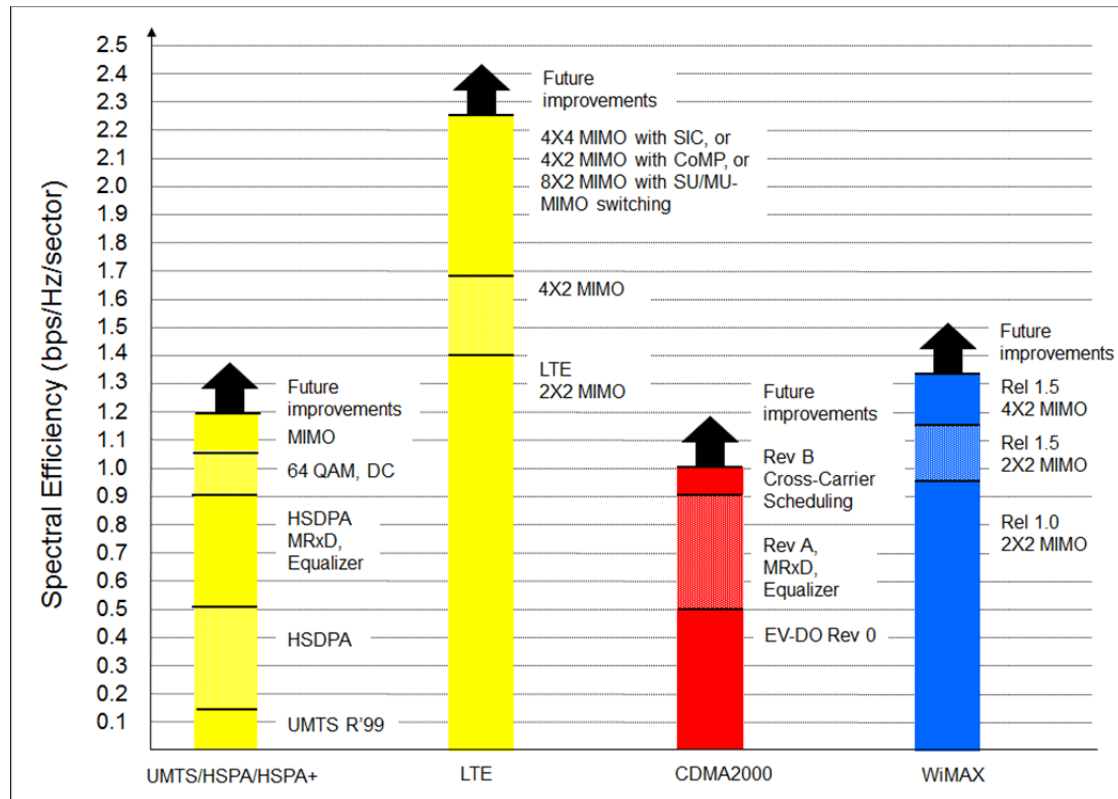
Figure 1: Rysavy Research Downlink Spectral Efficiency Comparison
